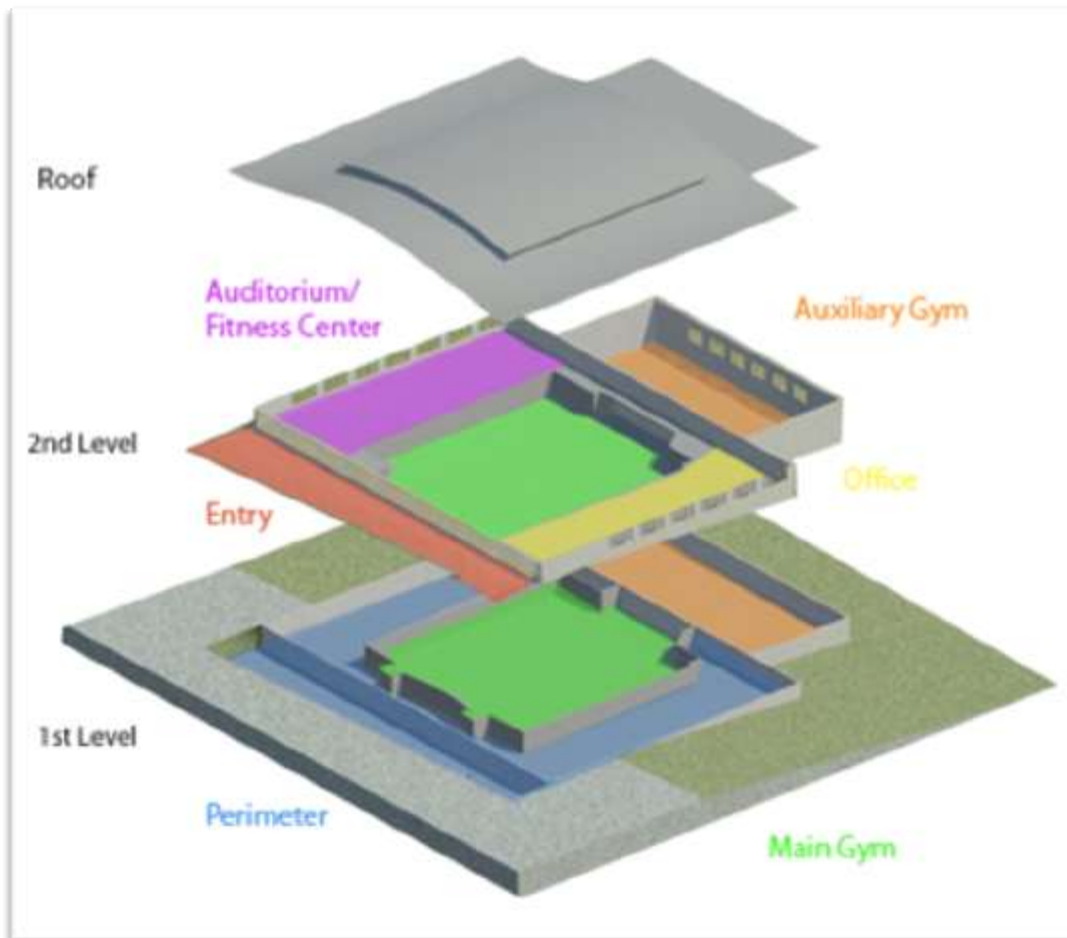
Exploded View
